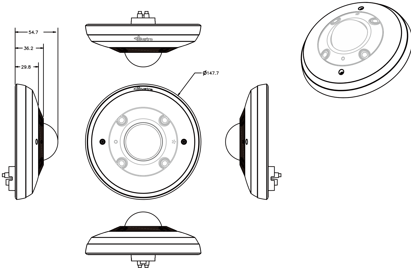
Illustra PRD Series 12MP Fisheye Indoor/Outdoor white TDN w/IR, WDR
